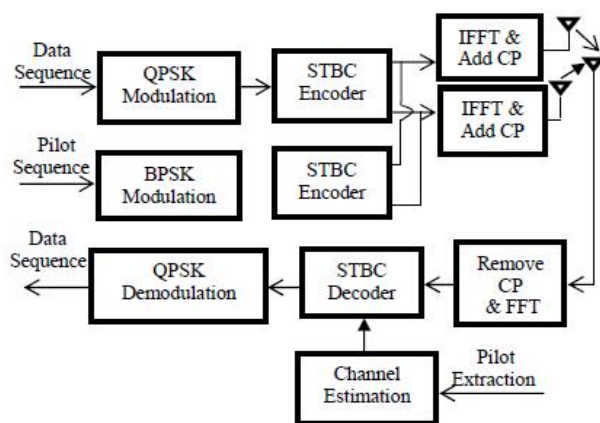
Figure 1 Block diagram of an STBC-OFDM system model
